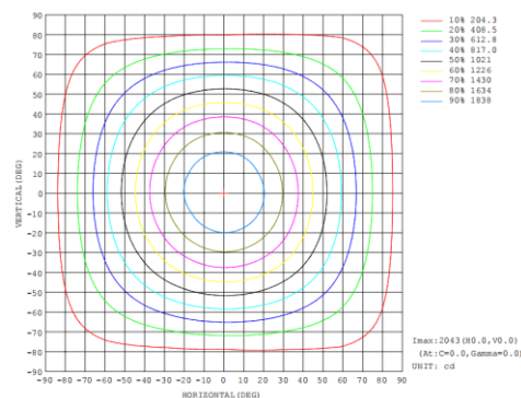
ISOCANDELA DIAGRAM
