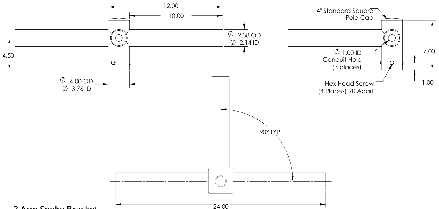
3 Arm Spoke Bracket at 90 Degree
